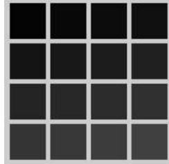
Figure 14. Residual Error
