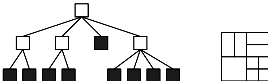
Figure 8. Tree Structure
