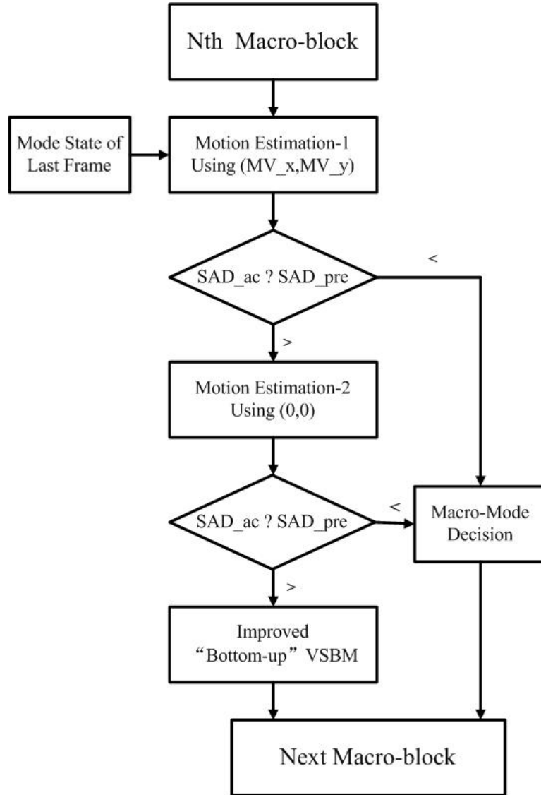
Figure 10. Prediction Flowchart
