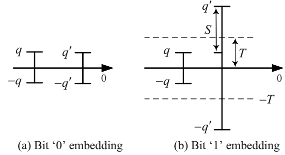
Figure 2. Embedding Model of HDC Embedding Method
