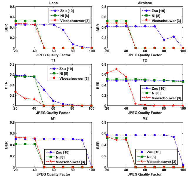
Figure 4. Robustness Comparison
